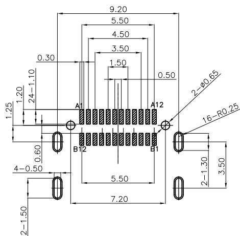
RECOMMENDED PCB LAYOUT (COMPONENT SIDE)
